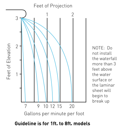
WATER FLOW REQUIREMENT CHART
